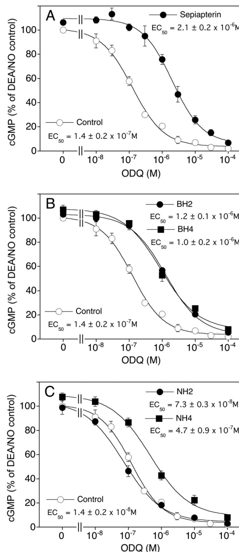
Fig. 5. Effect of pteridine supplementation on NO-induced cGMP accumulation in ODQ-treated endothelial cells. Endothelial cells were pretreated in culture medium for 24 h in the absence (control) or presence of 0.1 mM sepiapterin (A) for 1 h with 0.1 mM BH2 or BH4 (B) or for 1 h with 0.1 mM NH2 or NH4 (C). Then cells were washed and preincubated in assay buffer for 15 min with increasing concentrations of ODQ, and cGMP formation was determined in response to 1 \mu M DEA/NO. Data are mean values \pm S.E.M. of three to five independent experiments.
